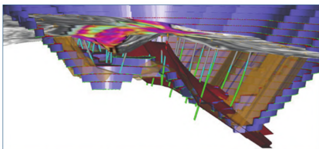
Sectional view of a surface showing draped mineralized zones, with 3D shear structure and coloured drillhole traces within an open pit design.
