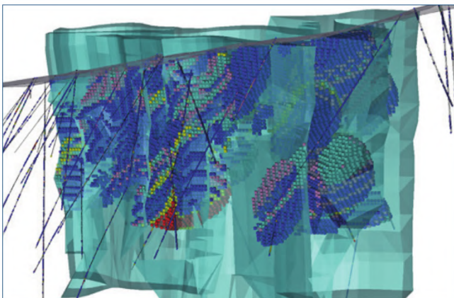
GEMS showing complex geological solid and block modelling based on drillhole and topographic mapping.
